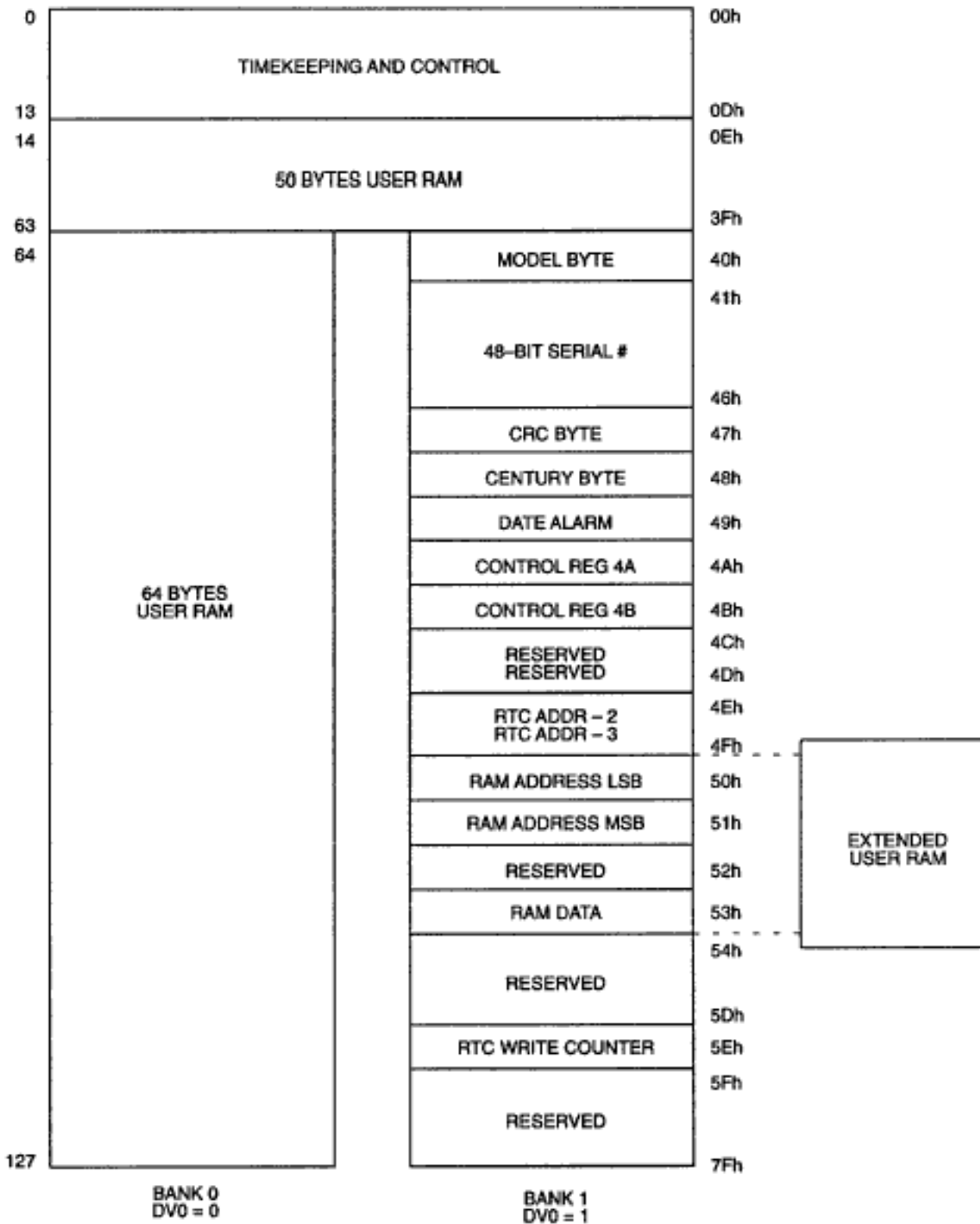
Figure 1. Register Block Partition
